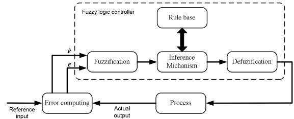
Figure 4. Fuzzy logic controller
